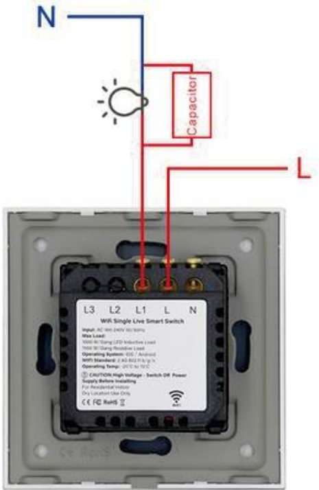
Wiring Diagram
